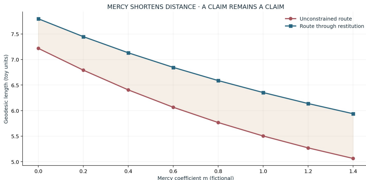
Figure 23. Mercy strength changes path length while the restitution condition persists
