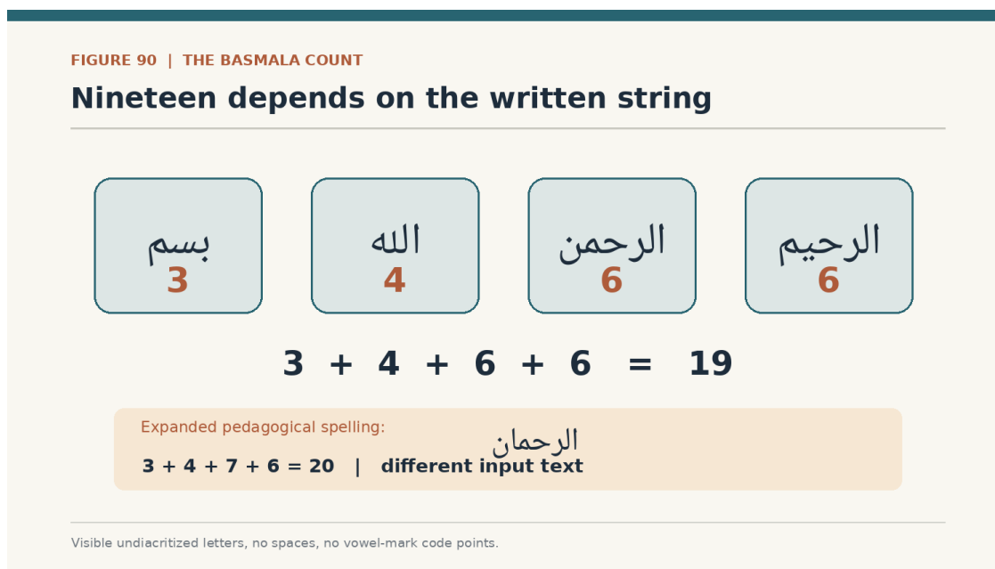
Figure 90. The familiar undiacritized basmala counts to nineteen letters; an explicitly changed pedagogical spelling counts to twenty.
