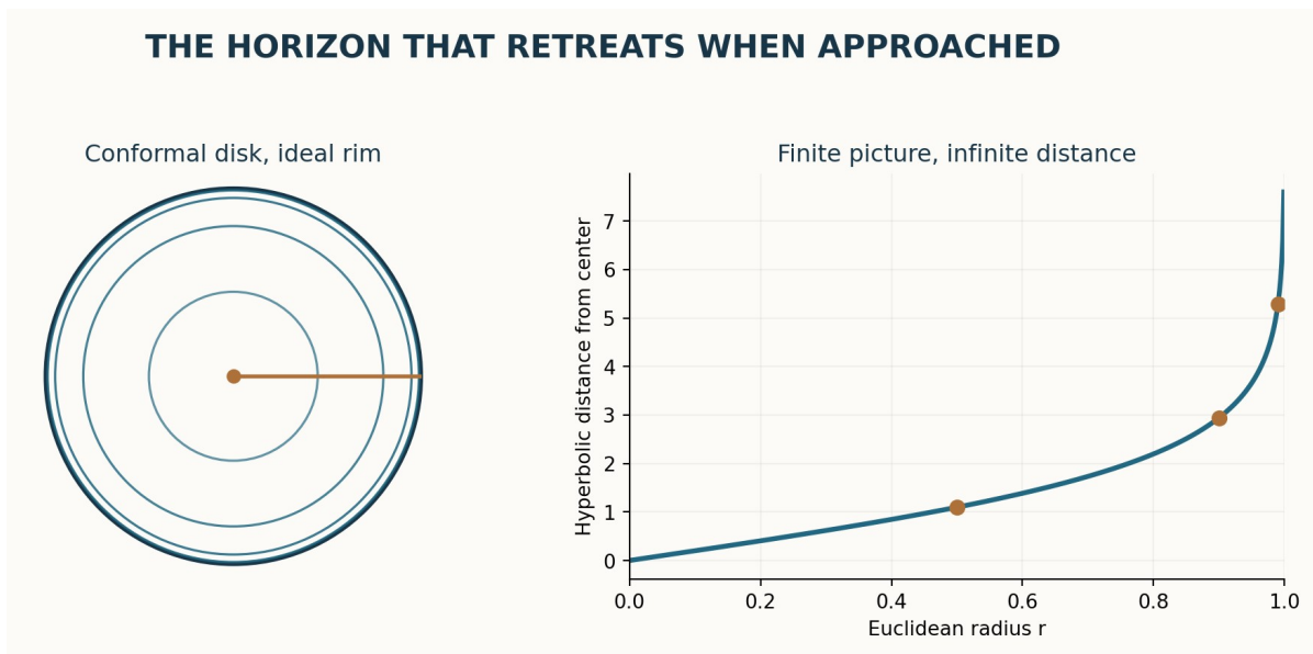
Figure 46. The Poincaré disk and its diverging radial distance to the ideal boundary
