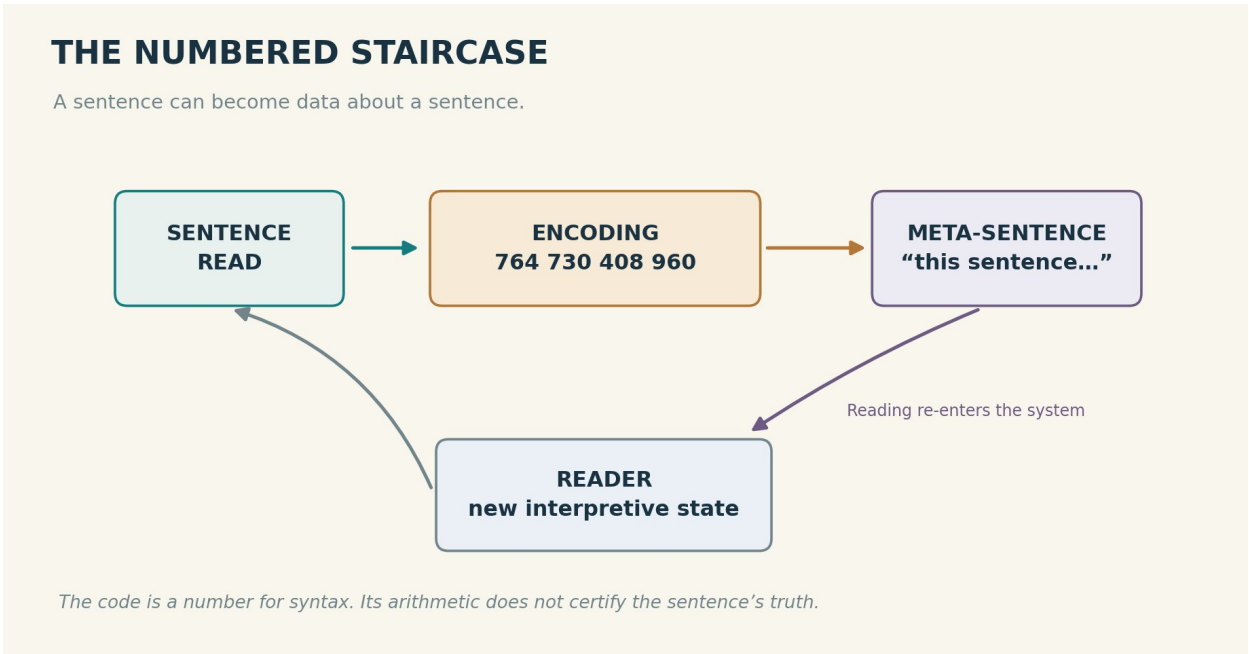
Figure 11: Syntax converted into Gödel code and sent back to interpretation
