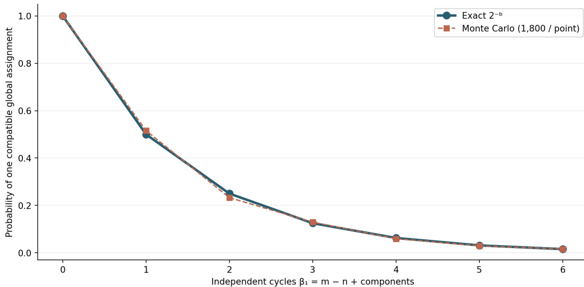
Figure 85. The exact cycle-rank law against seeded Monte Carlo over eight-variable graphs.
