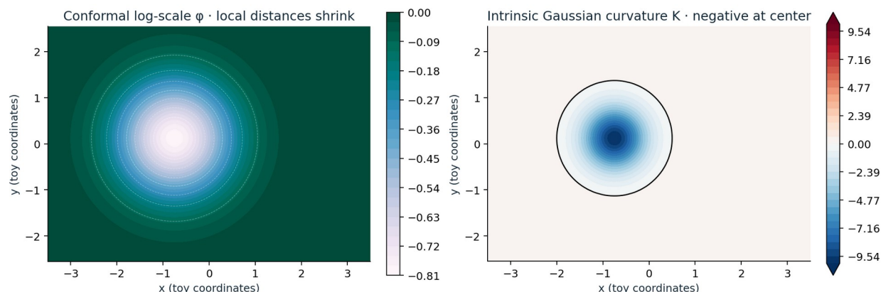
Figure 21. The metric's scale factor and its actual Gaussian curvature
