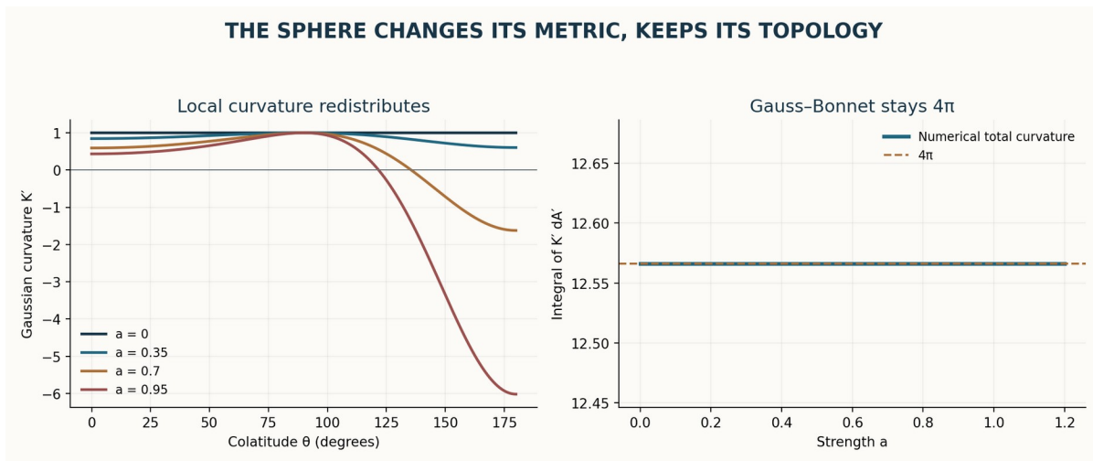
Figure 47. Local curvature changes under conformal rescaling while Gauss–Bonnet keeps total curvature equal to four pi
