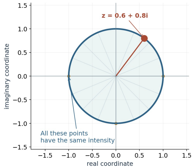
Figure 64. One intensity reading is compatible with every phase on a full circle in the complex plane
