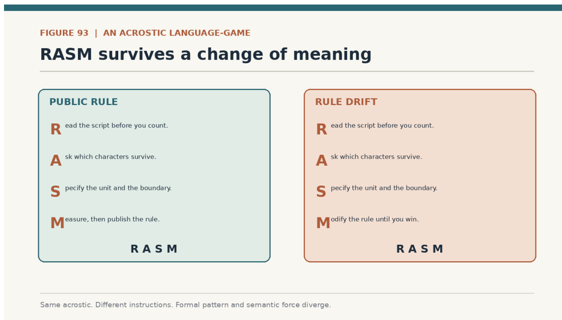
Figure 93. An acrostic remains RASM even when the meaning of the final instruction changes.
