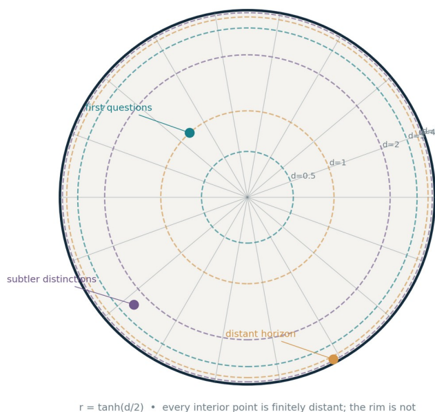
Figure 9: The Poincaré disk as a horizon for finite interpretation
