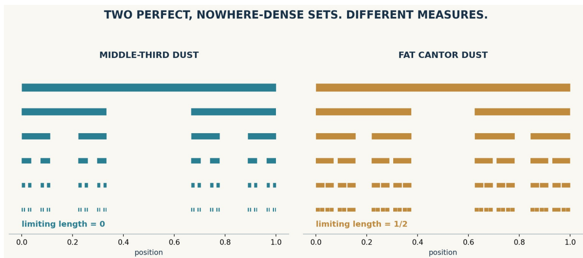
Figure 49. Middle-third dust and fat Cantor dust: two nowhere-dense constructions with different limiting lengths
