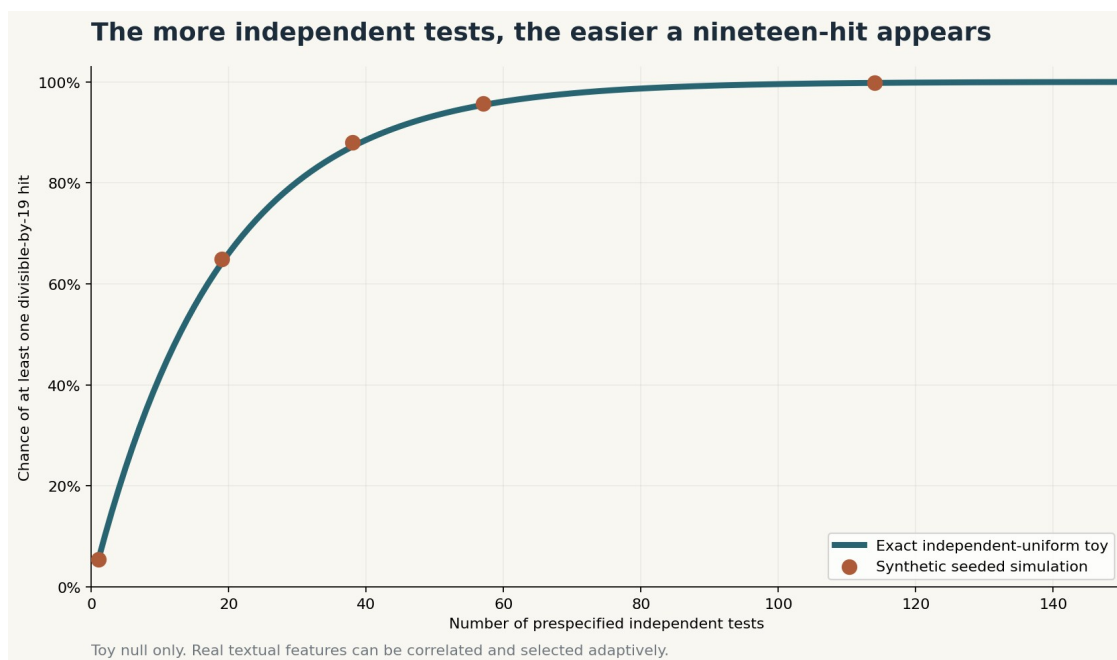
Figure 91. Multiple-testing pressure in a synthetic independent-uniform model, with a seeded numerical check.
