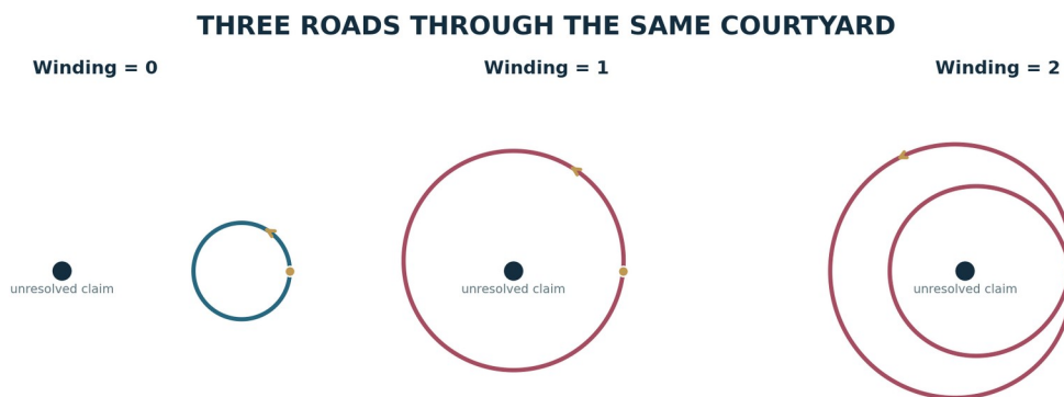
Figure 25. Three loops around an unresolved claim carry different winding numbers
