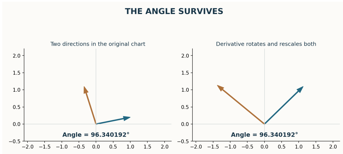
Figure 45. The preserved angle between two vectors under the derivative of a conformal map
