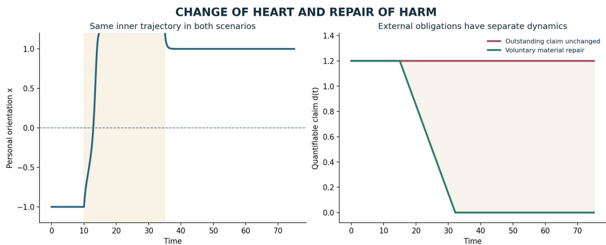
Figure 29. A changed habit and an outstanding claim evolve on separate axes
