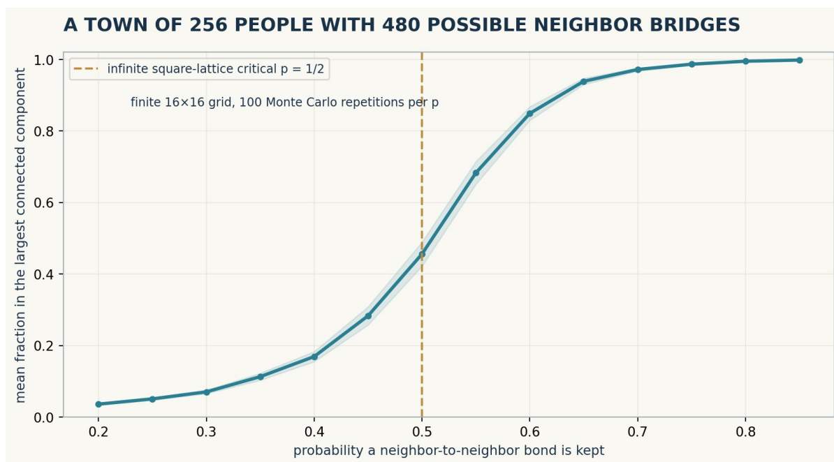
Figure 52. Monte Carlo sweep of nearest-neighbor connectivity in a finite square town; the infinite-lattice threshold is marked for comparison
