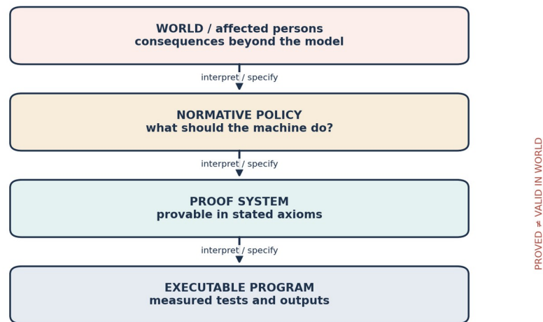
Figure 70. Object program, proof system, policy specification, and world are distinct levels
