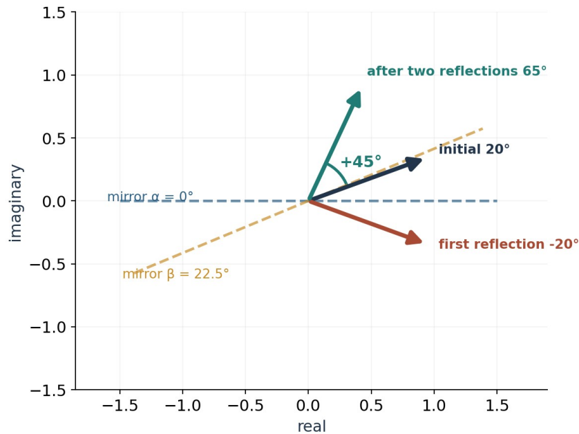
Figure 68. Two reflections rotate a complex signal by twice the angle between their reflecting axes
