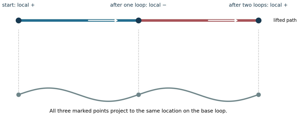
Figure 16. The orientation double cover: a label swaps after one circuit and returns after two
