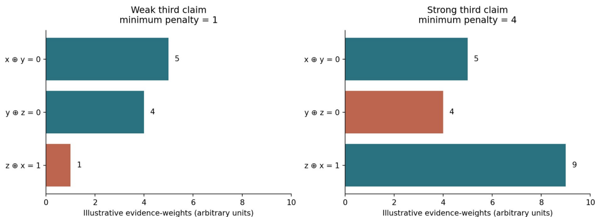
Figure 86. The chosen minimal repair changes when the arbitrary evidence weights change.
