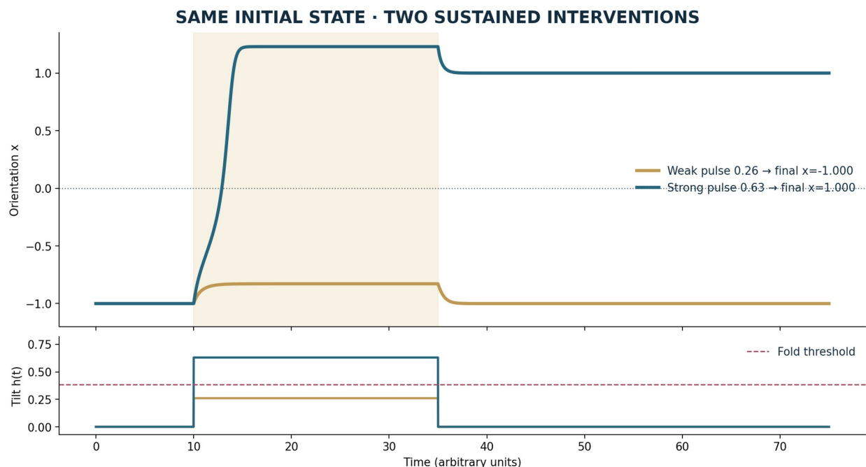
Figure 28. A weak pulse and a sufficiently strong pulse lead to different final basins
