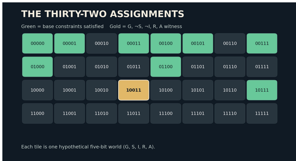
Figure 76. The five-predicate Boolean palace: ten of thirty-two assignments obey the stipulated base constraints; the gold tile is an open countermodel.
